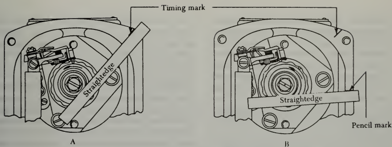
FIGURE 4-44. Aligning straightedge.
